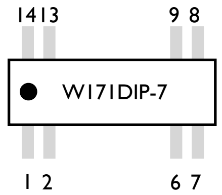
Reed switch chip top view
