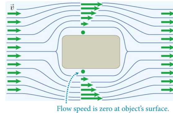
(b) Low flow speed, nonzero viscosity
