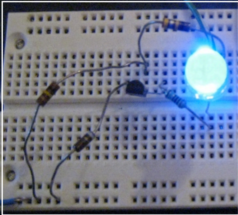
Current source
